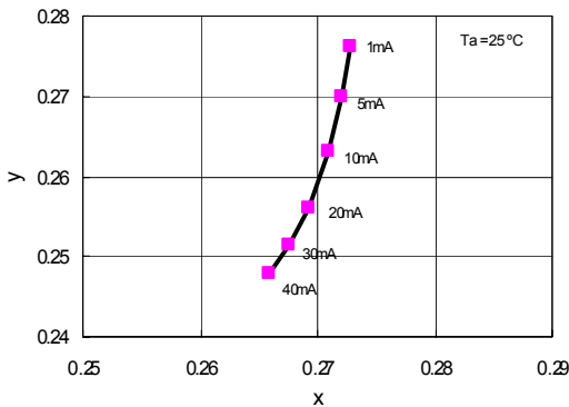
Forward Current VS. Chromaticity coordinate
