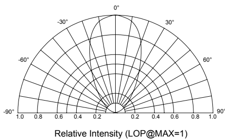
Beam Pattern
