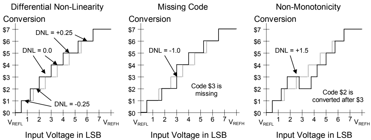
Figure 3. Differential Non-Linearity, Missing Codes, and Non-Monotonicity Graphs
